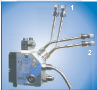
Vertical (1) and horizontal (2) positions for air inputs
